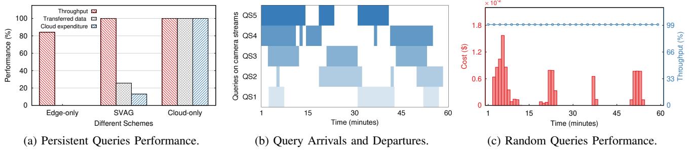
Fig. 5: Performance under different query patterns. The transferred data and cloud expenditure values in (a) are normalized by that of the Cloud-only scheme, and the throughput values are calculated by averaging across all queries. The colored time windows in each row of (b) indicate the existence of queries on a specific camera stream. (c) assumes it costs $0.1 to transfer 1 GB data between the edge node and the cloud and sums up the money paid for data transfer and cloud expenditure to obtain the cost values.
