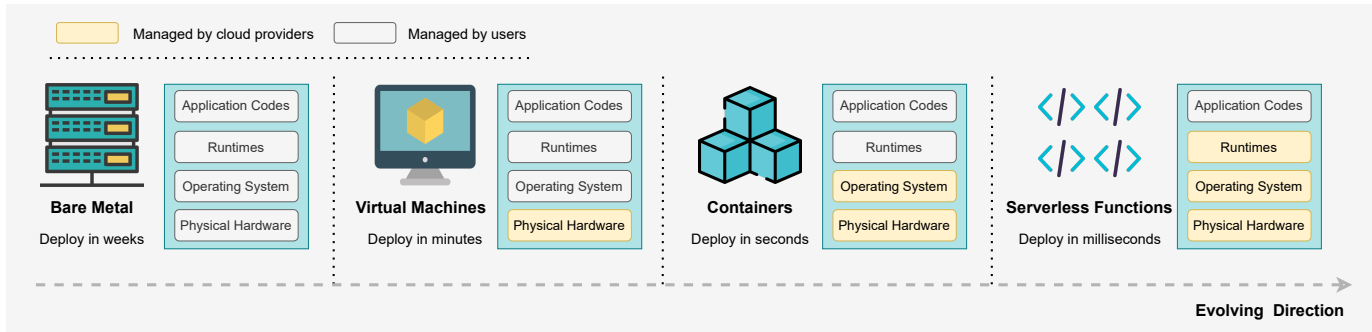
Fig. 2: The evolution of application deployment architecture. Users take diminishing responsibilities and can focus on the development of application codes with serverless computing. The increasingly lightweight virtualization technologies significantly improve the development and deployment speeds, agility, portability, and time-to-market.
