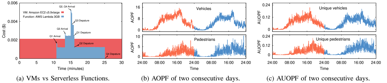
Fig. 3: Video analytics statistics on real-world camera streams. (a) The respective costs of using VMs and serverless functions to answer randomly generated object detection queries on 4 video streams (Q1-Q4) in 30 minutes. (b) and (c) depict the corresponding average objects per frame (AOPF) and average unique object per frame (AUOPF) for querying the number of vehicles (top) and pedestrians (bottom) on a crossroad camera stream.
