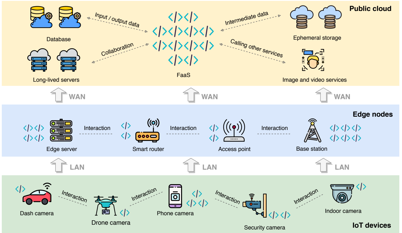
Fig. 4: An overview of SVAG. There are three hierarchies in this framework, from IoT devices with cameras and onboard computing resources, to heterogeneous resource-constrained edge nodes, to the resource-rich public cloud. Serverless functions are the smallest unit of configuration and placement. Interactions and collaborations within and between hierarchies are enabled for the geo-distributed execution of a serverless video analytics pipeline.
